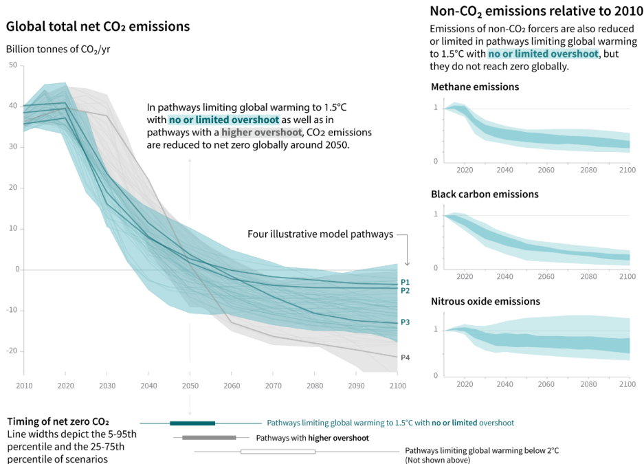
Figure B: Global emissions pathways
